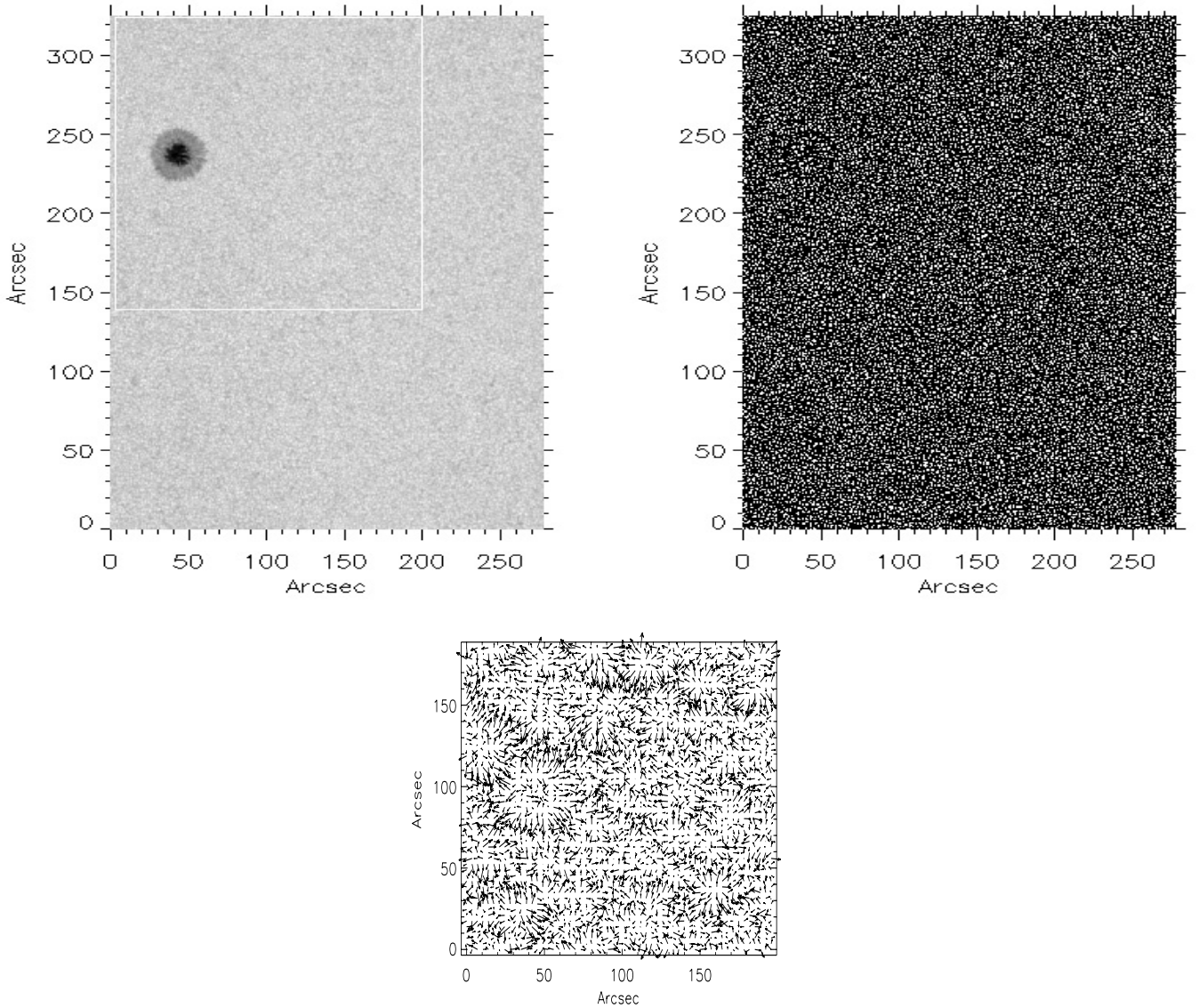
Fig. 2. Close-up view of the field around a spot as delineated in Fig. 1 ( top left ) with its segmentation ( top right ). Below, resulting velocity field from granule tracking (note the clear signature of the moat flow associated with the spot near x = 50 , y = 100 ).
